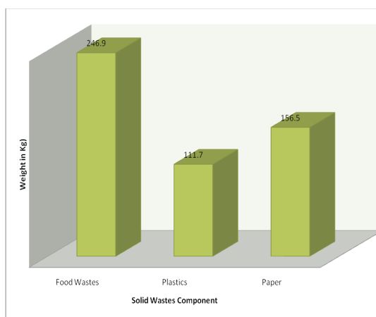
Figure 3: Mean weekly weight of the recyclable solid wastes components most highly generated at the three locations
