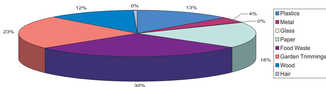
Figure 4: Percentage monthly total recyclable solid wastes components generated at the three locations
